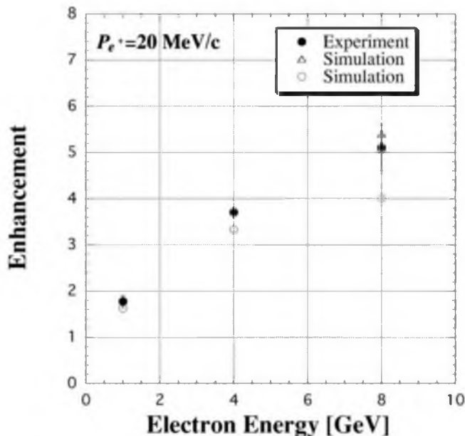
FIG. 5. Incident electron-energy dependence of the positron-yield enhancement at P_{e^+} = 20 MeV/c for the 2.2-mm-thick tungsten monocrystalline target. The open circles and triangle show the simulation result by our code [see the text (Sec. III B) for details] and by Baier and Strakhovenko [19], respectively.
