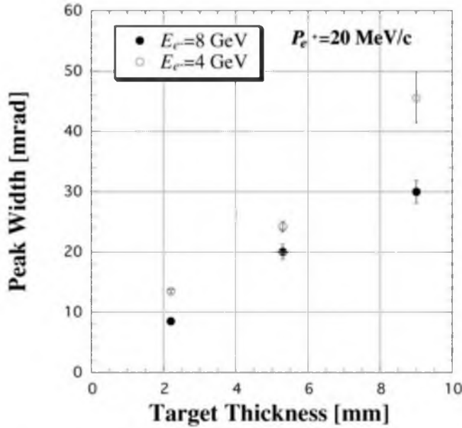
FIG. 3. Variations in the peak width of the rocking curve at P_{e^+} = 20 MeV/c for E_{e^-} = 4 and 8 GeV as a function of the target thickness.
