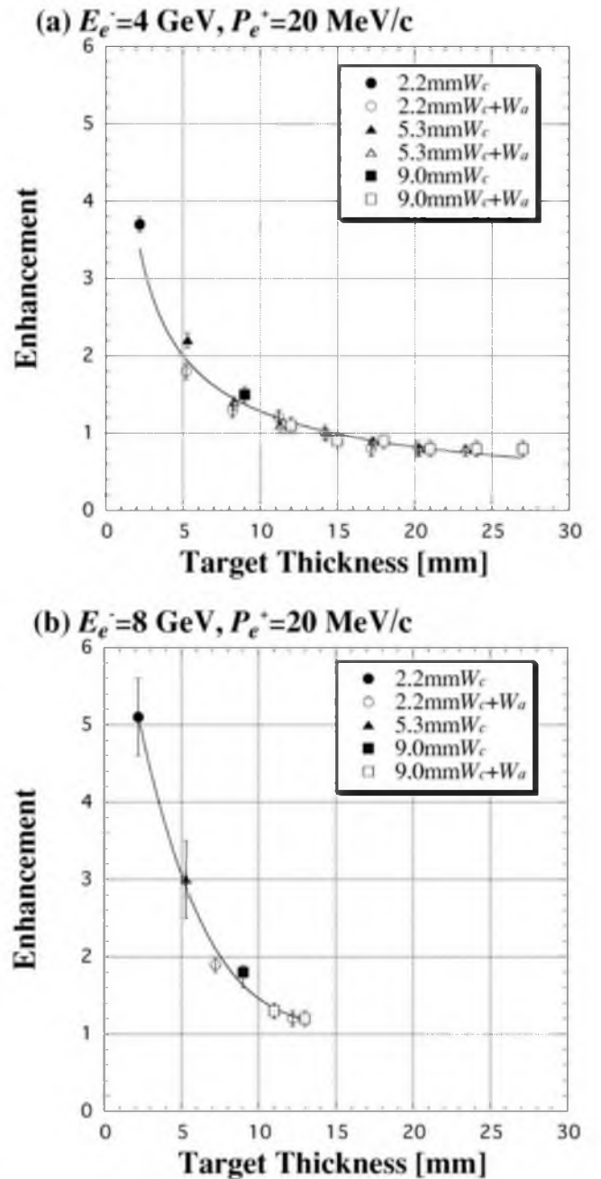
FIG. 4. Variations in the enhancement of the positron yield at P_{e^+} = 20 MeV/c for (a) E_{e^-} = 4 GeV and (b) E_{e^-} = 8 GeV as a function of the target thickness. The solid curves drawn through the data are only to guide the eye.
