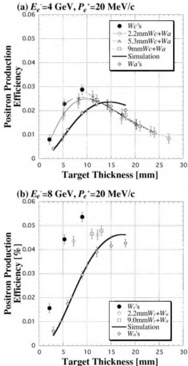
FIG. 6. Positron production efficiencies measured for the crystal and combined targets at P_{e^+} = 20 \text{ MeV}/c for (a) E_{e^-} = 4 \text{ GeV} and (b) E_{e^-} = 8 \text{ GeV} . The thick solid curves drawn through the data obtained for the W_a 's are based on a simulation. The other thin curves drawn through the data are only to guide the eyes.
