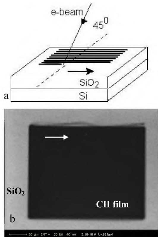
Figure 1 a- Fabrication of CH film. The raster of e-beam on SiO 2 surface by oblique incidence. b- The REM image of CH film on SiO 2 . The arrows in (a) and (b) point to the direction of e-beam movement.
