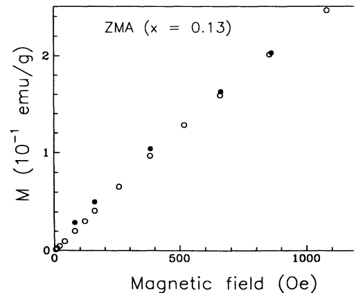
FIG. 7. Part of the hysteresis curve of ZMA with x=0.13 , measured at 103 K with increasing (open symbols) and decreasing (solid symbols) the field.
