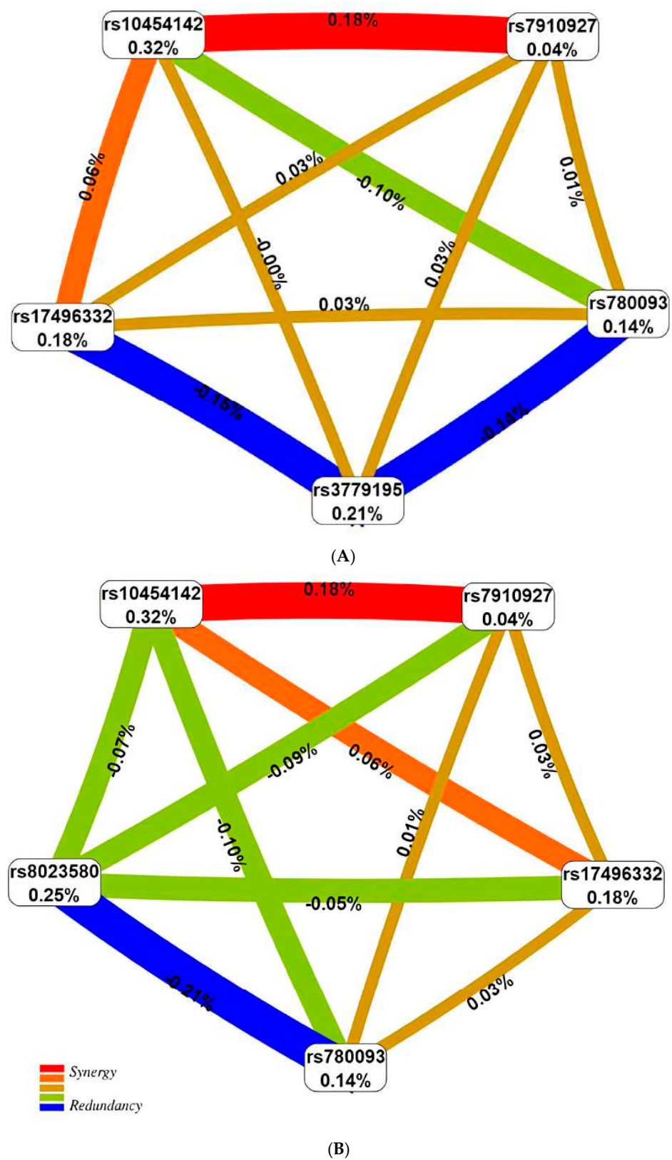
Figure 1. The entropy graph of the five loci models of SNP \times SNP interactions associated with breast cancer based on the MDR analysis: Model 1 (A) (Wald st. = 51.58, p = 6.88 \times 10^{-13} , p_{\text{perm}} < 0.001 ), Model 2 (B) (Wald st. = 47.77, p = 4.78 \times 10^{-12} , p_{\text{perm}} < 0.001 ). The red and orange colors denote strong and moderate synergism, respectively, brown color denotes the independent effect, green and blue colors denote moderate and strong antagonism, respectively.
